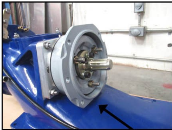
Option 1 HJ212 Close Coupling
